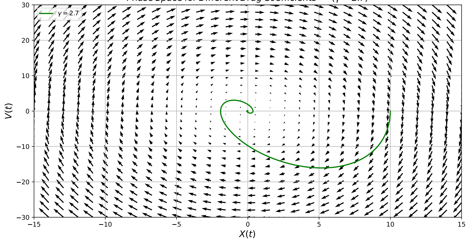
Phase Space for Different Drag Coefficients – ( \gamma = 2.7 )
